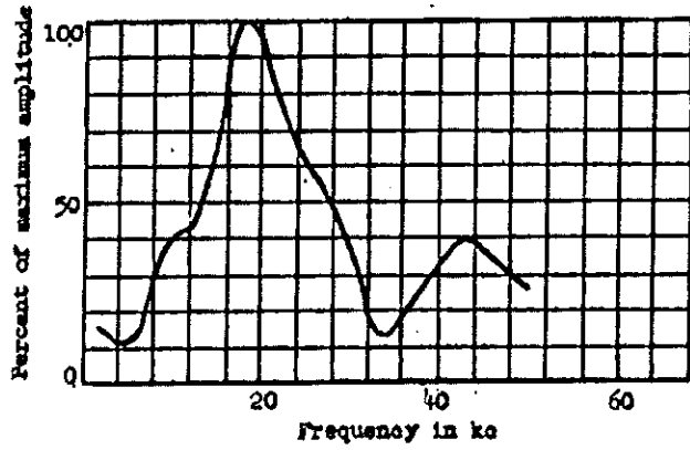
Fig. 3.89 Frequency function of broadband pulse Shot No. 10 1000 km from ground zero
